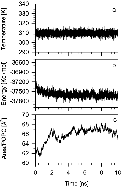
FIGURE 2 Diagrams showing the time development of the temperature ( a ), potential energy ( b ), and surface area per POPC headgroup ( c ) in the POPC-LA bilayer. The equilibrium average surface area is 66 \pm 1 \text{ Å}^2 .
